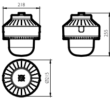
GreenUp Wellglass BY200P
